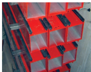
Storing stop logs on site
